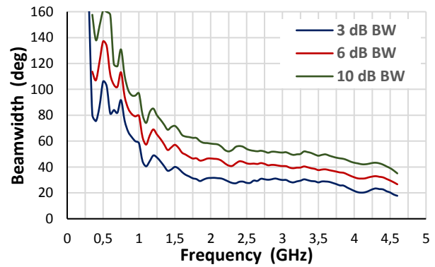
H plane
